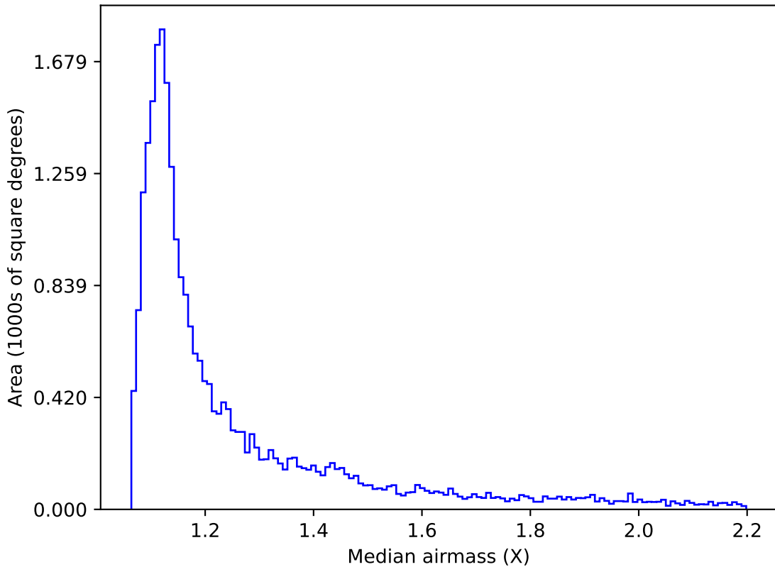
weather_cloudso6v3.4_10yrs Yr 1 i band: Median airmass
