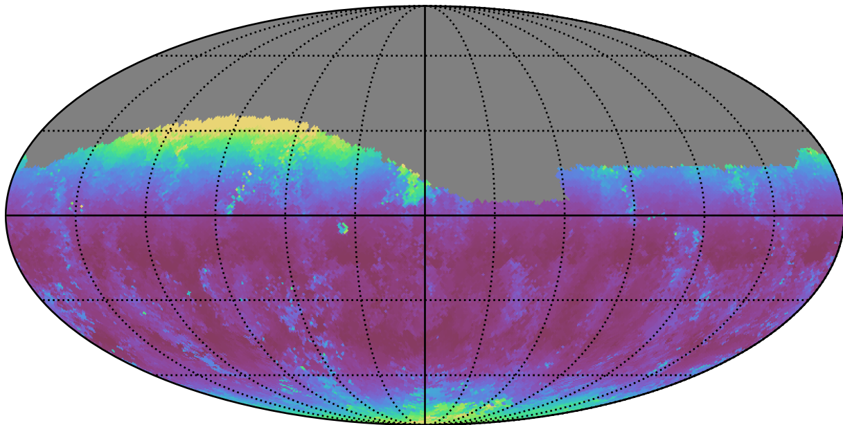
weather_cloudso6v3.4_10yrs Yr 1 g band: Median airmass
