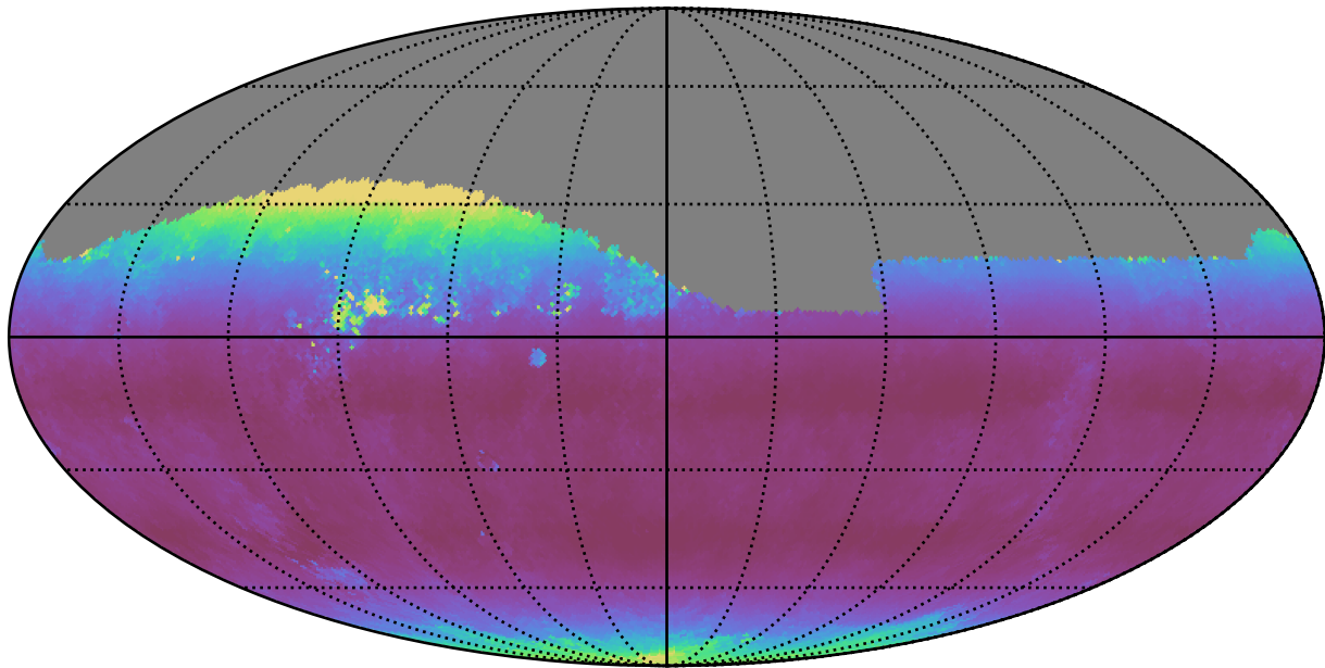
weather_cloudso6v3.4_10yrs Yr 1 all bands: Median airmass
