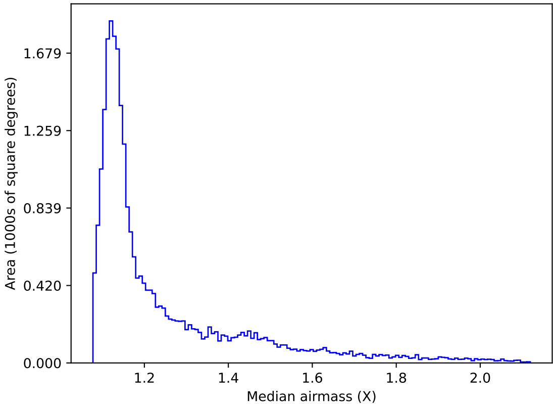
weather_cloudso6v3.4_10yrs Yr 1 all bands: Median airmass
