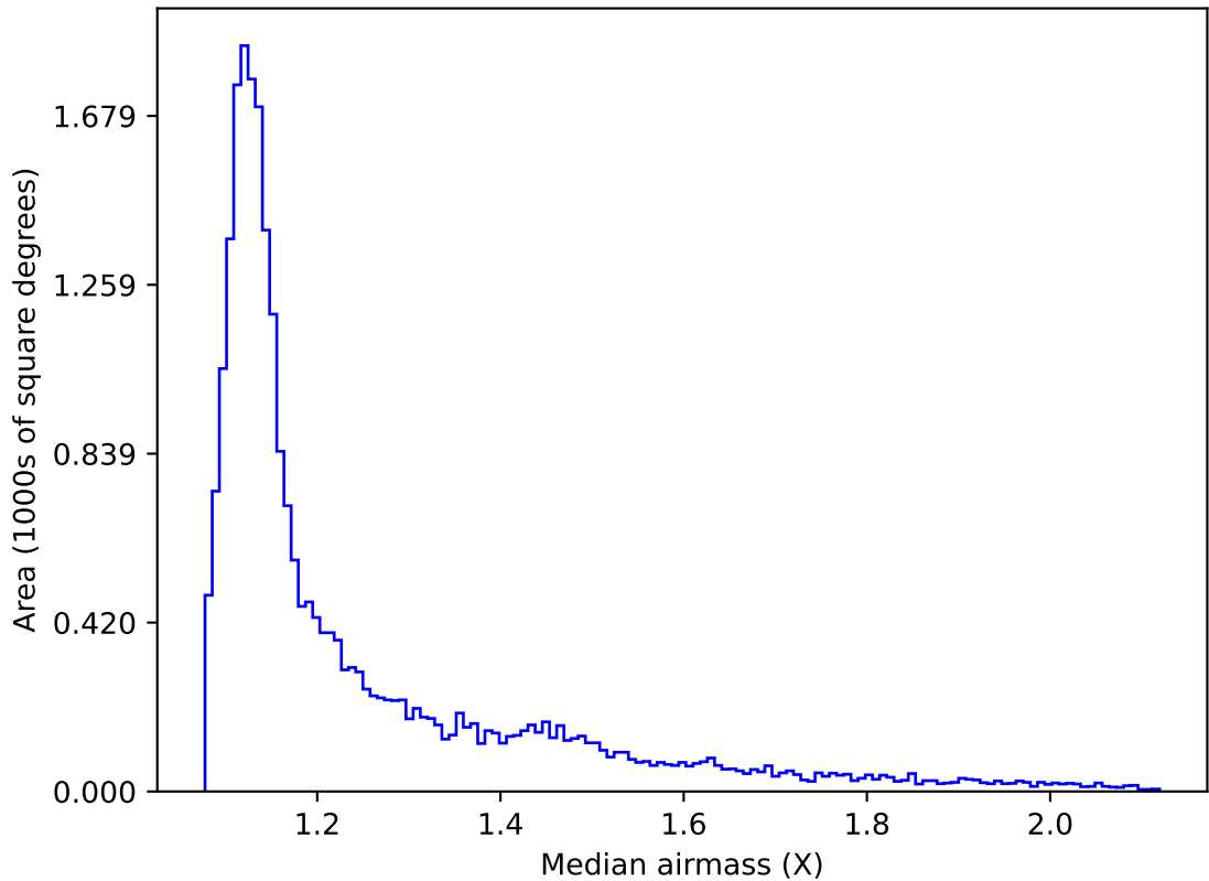
weather_cloudso6v3.4_10yrs Yr 1 all bands: Median airmass
