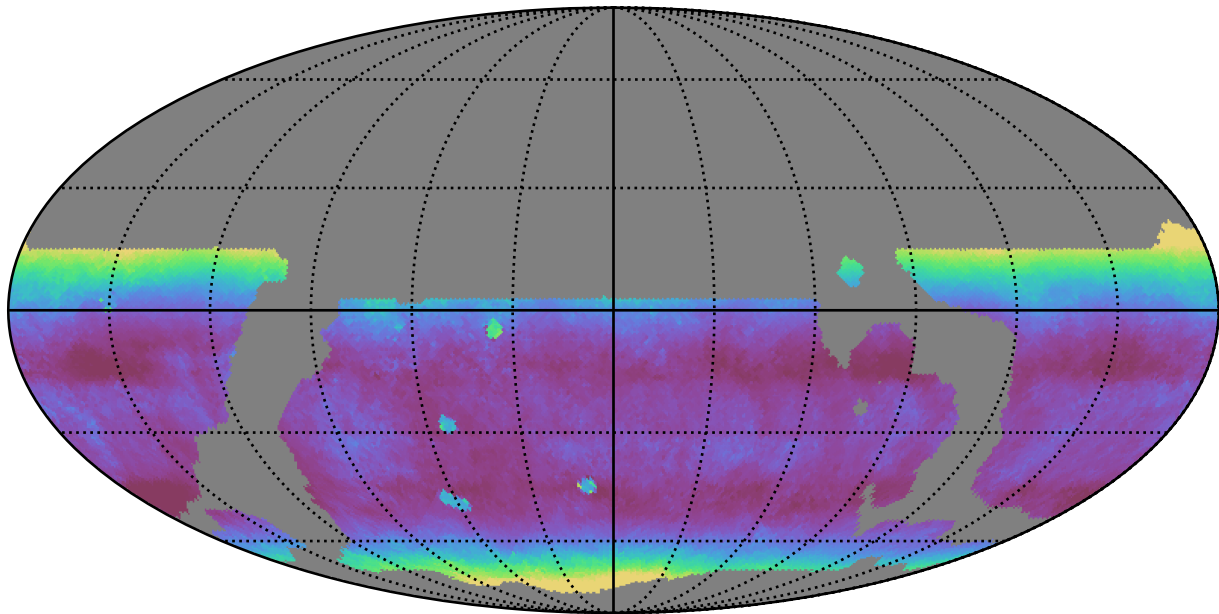
weather_cloudso6v3.4_10yrs WFD z band: Median airmass
