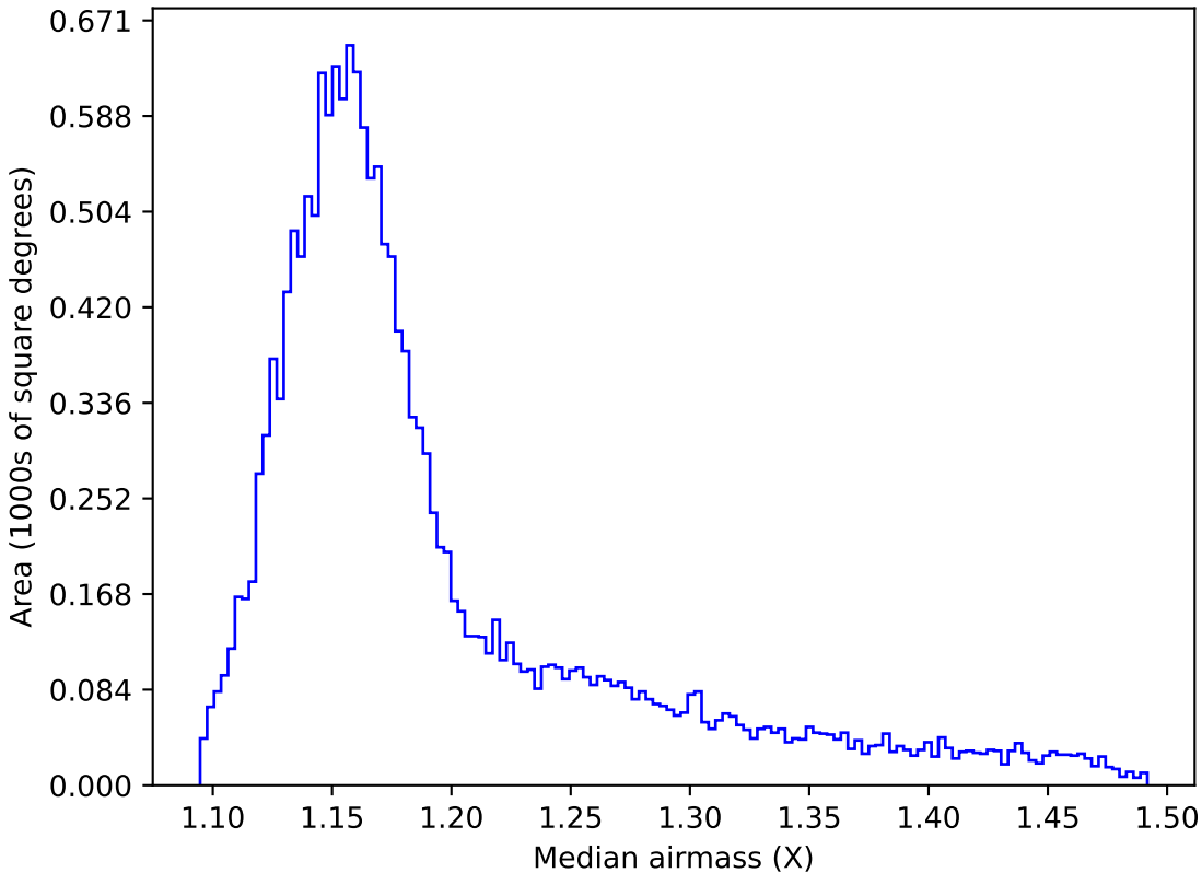
weather_cloudso6v3.4_10yrs WFD z band: Median airmass
