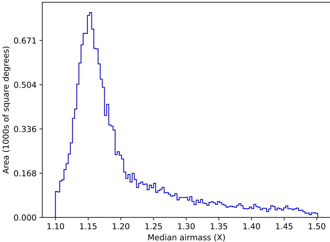
weather_cloudso6v3.4_10yrs WFD y band: Median airmass
