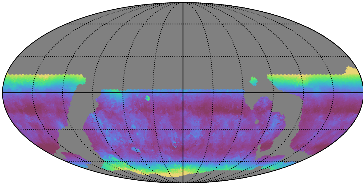
weather_cloudso6v3.4_10yrs WFD u band: Median airmass
