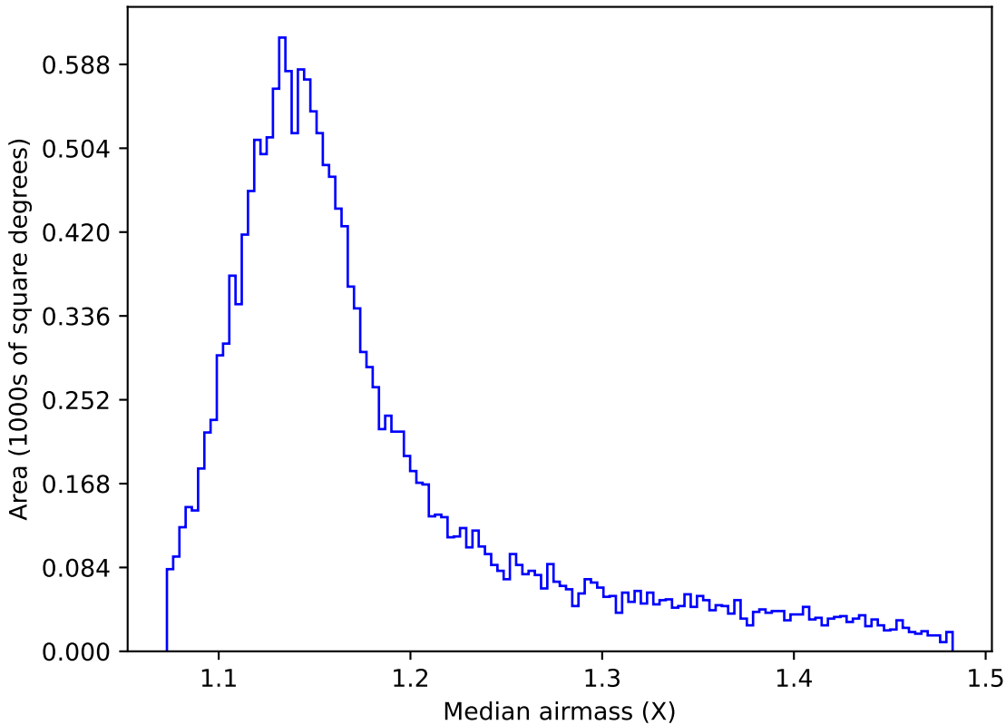
weather_cloudso6v3.4_10yrs WFD u band: Median airmass
