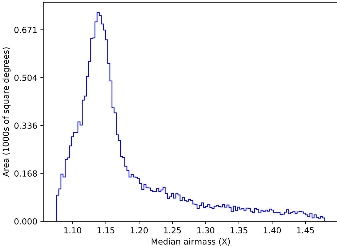
weather_cloudso6v3.4_10yrs WFD r band: Median airmass
