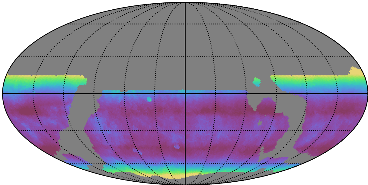
weather_cloudso6v3.4_10yrs WFD i band: Median airmass
