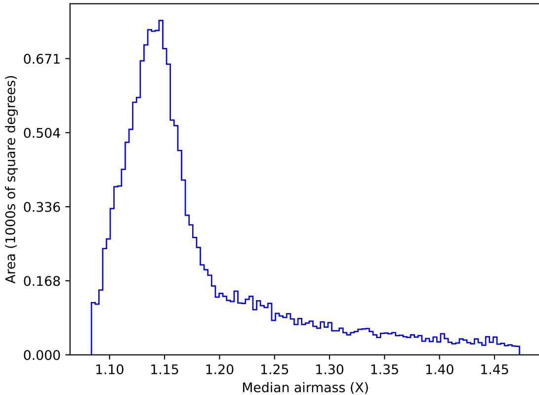
weather_cloudso6v3.4_10yrs WFD i band: Median airmass
