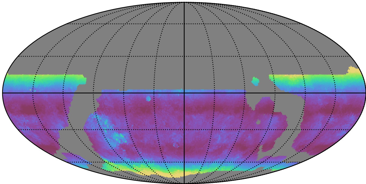
weather_cloudso6v3.4_10yrs WFD g band: Median airmass
