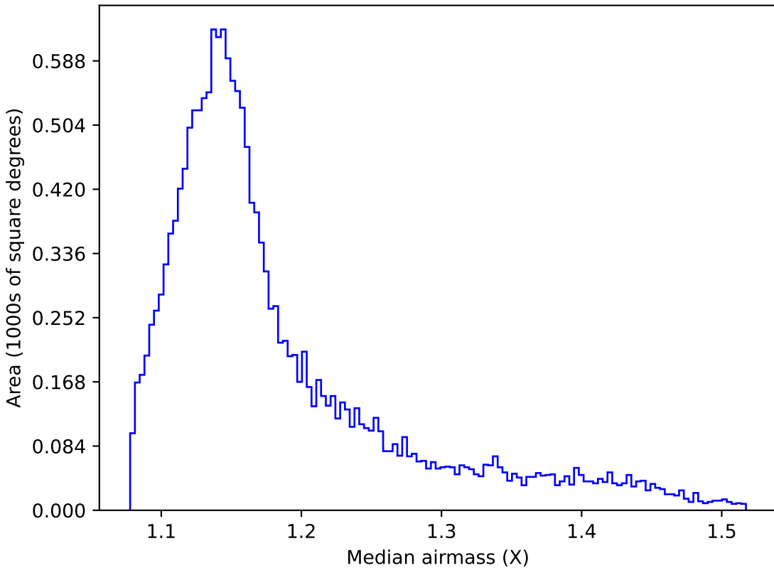
weather_cloudso6v3.4_10yrs WFD g band: Median airmass
