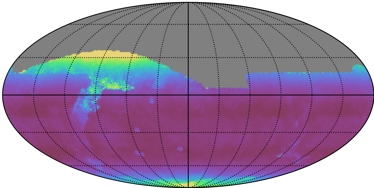
weather_cloudso6v3.4_10yrs All sky z band: Median airmass
