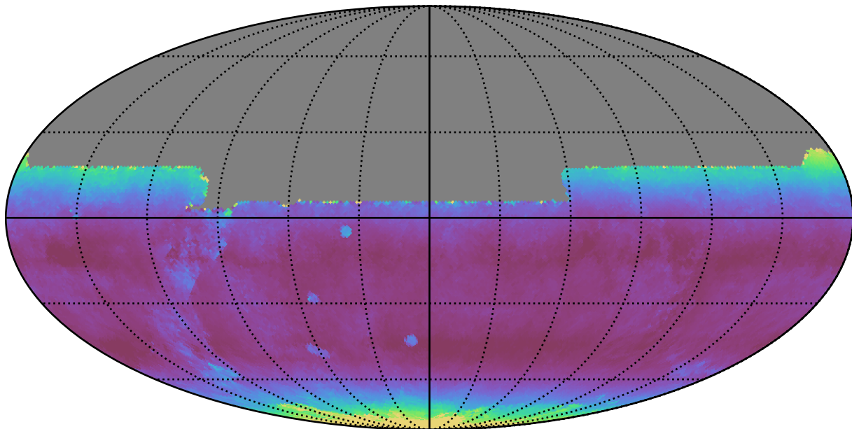
weather_cloudso6v3.4_10yrs All sky y band: Median airmass
