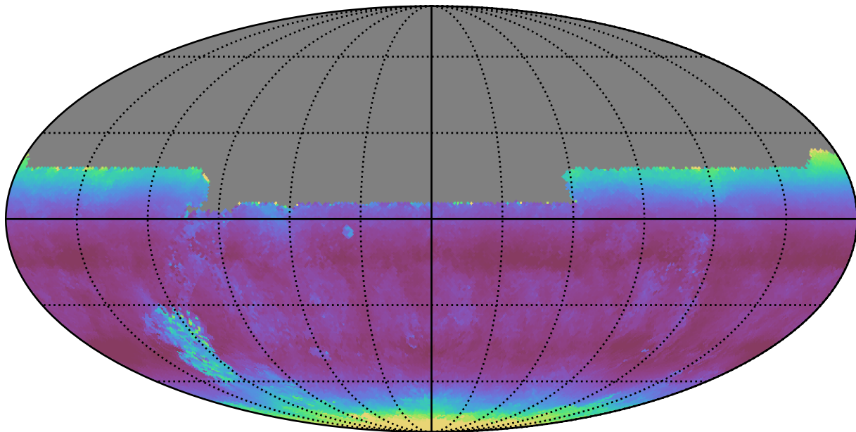
weather_cloudso6v3.4_10yrs All sky u band: Median airmass
