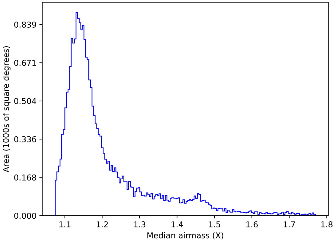
weather_cloudso6v3.4_10yrs All sky u band: Median airmass
