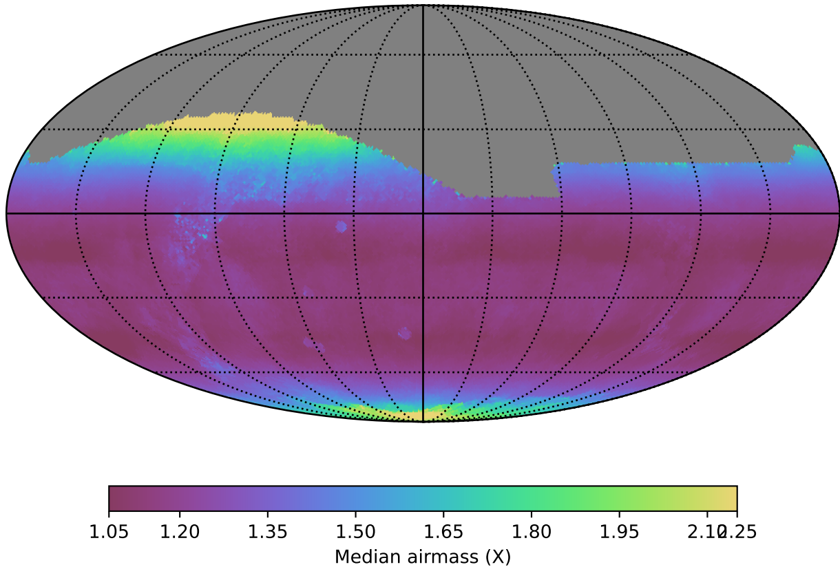
weather_cloudso6v3.4_10yrs All sky r band: Median airmass
