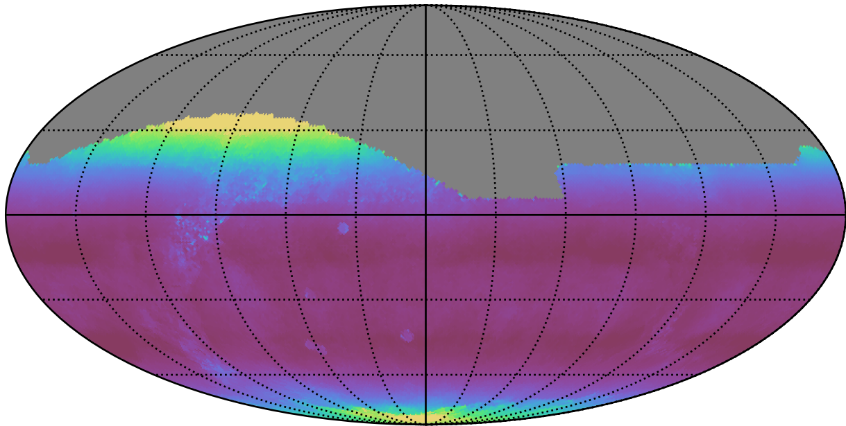
weather_cloudso6v3.4_10yrs All sky r band: Median airmass
