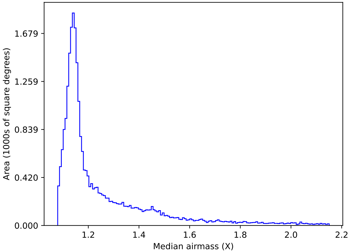
weather_cloudso6v3.4_10yrs All sky r band: Median airmass
