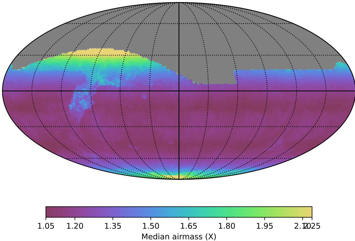
weather_cloudso6v3.4_10yrs All sky i band: Median airmass
