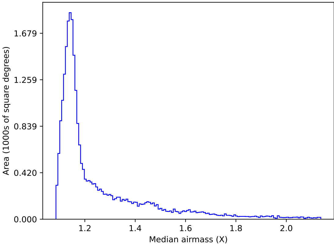
weather_cloudso6v3.4_10yrs All sky i band: Median airmass
