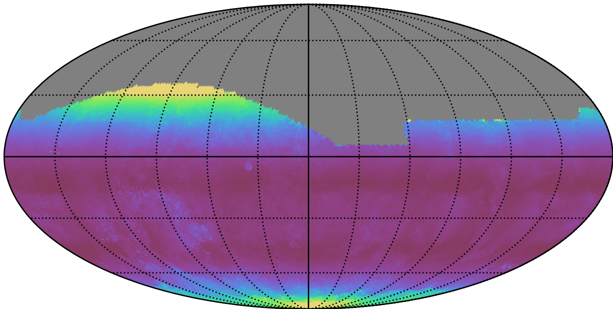
weather_cloudso6v3.4_10yrs All sky g band: Median airmass
