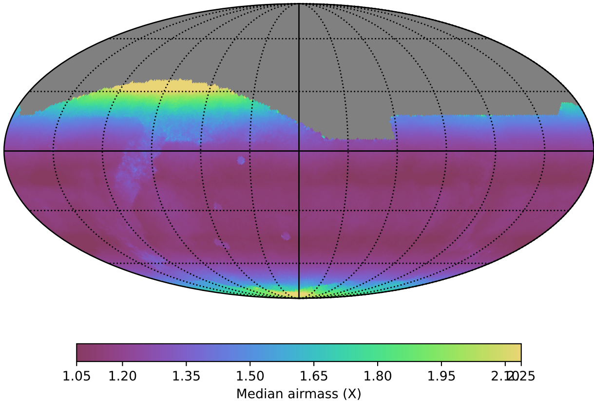
weather_cloudso6v3.4_10yrs All sky all bands: Median airmass
