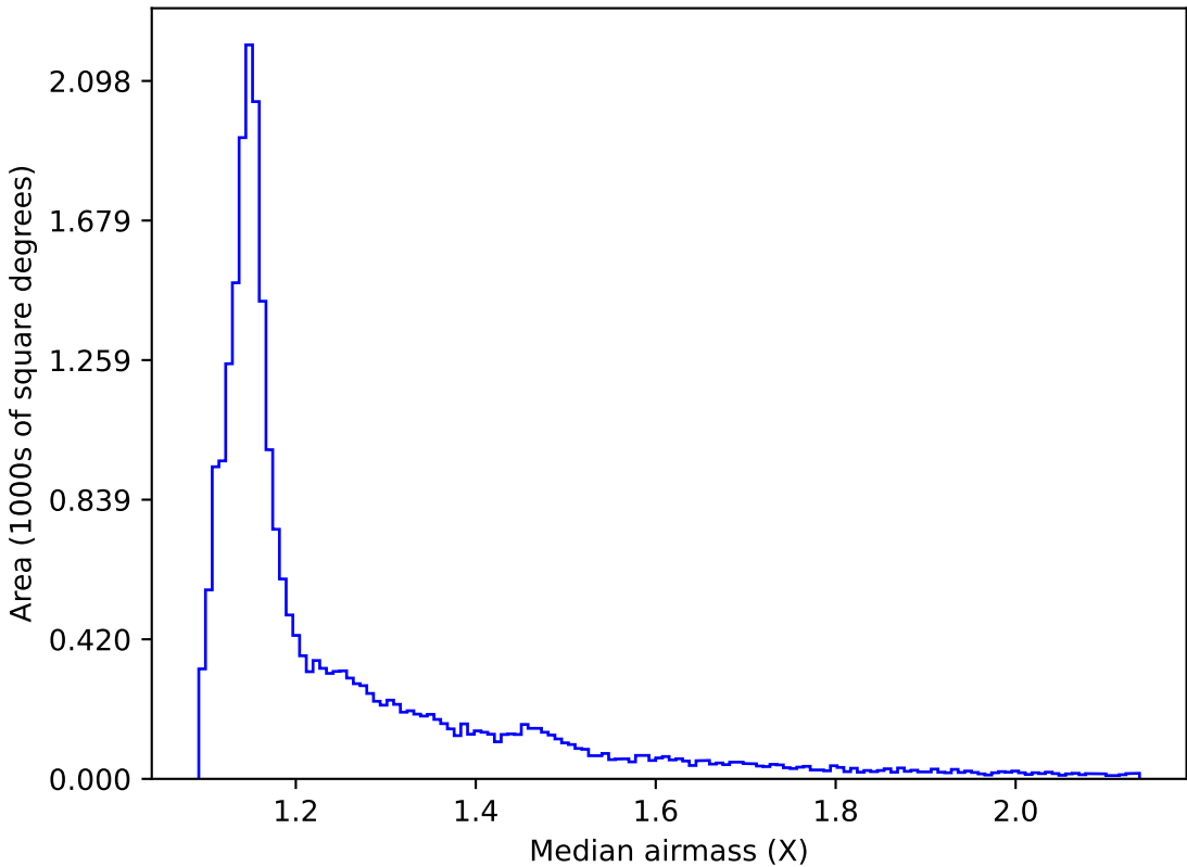
weather_cloudso6v3.4_10yrs All sky all bands: Median airmass
