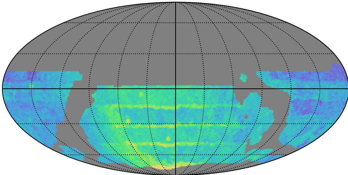
weather_cloudso6v3.4_10yrs WFD z band: Median Season Length
