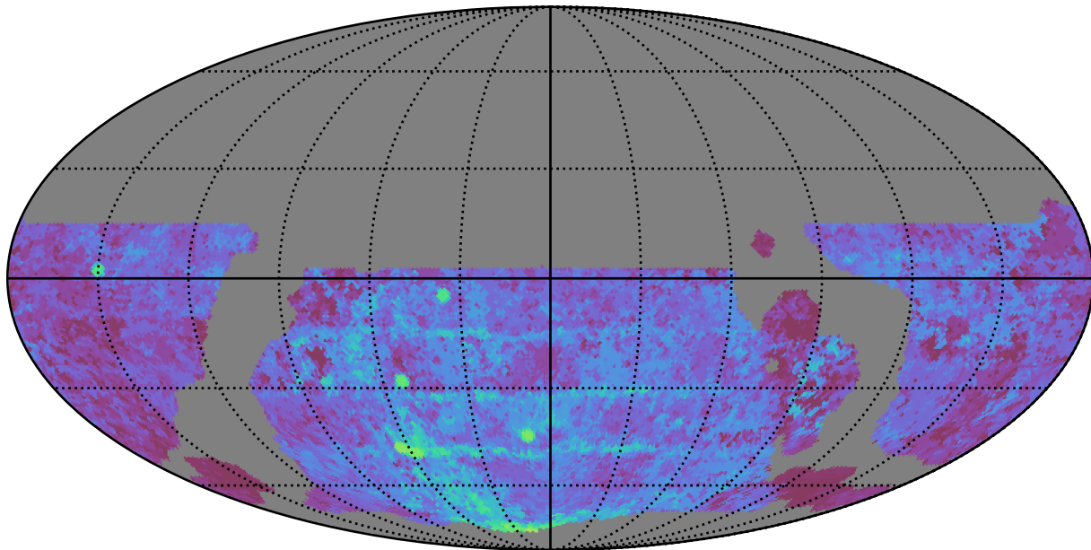
weather_cloudso6v3.4_10yrs WFD u band: Median Season Length
