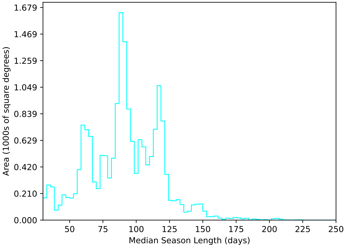
weather_cloudso6v3.4_10yrs WFD u band: Median Season Length
