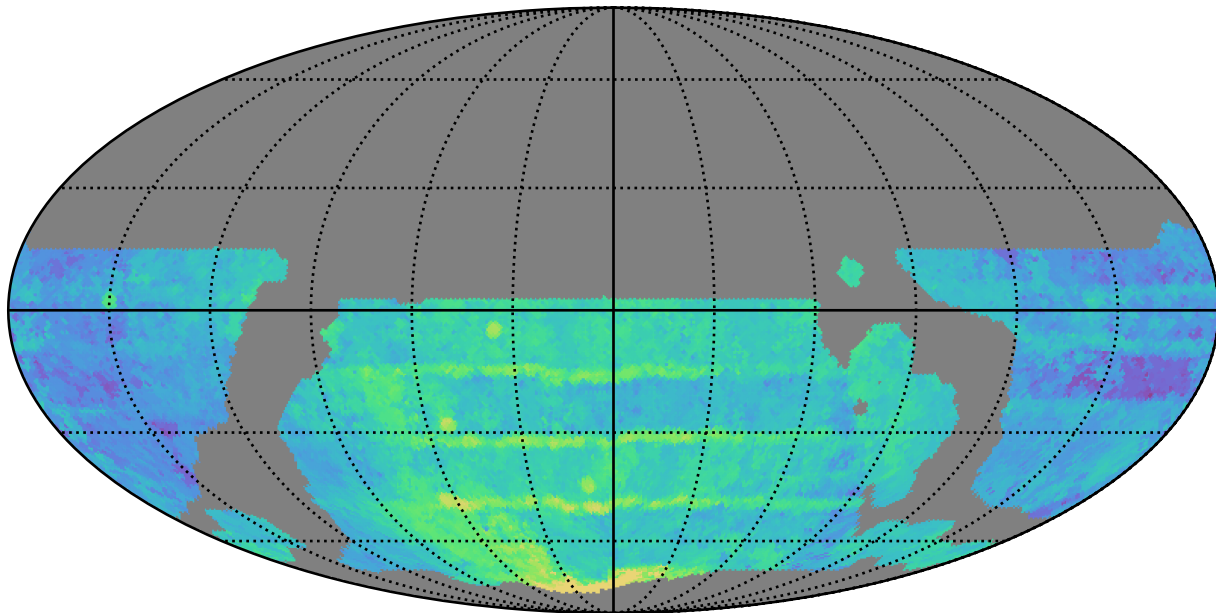
weather_cloudso6v3.4_10yrs WFD r band: Median Season Length
