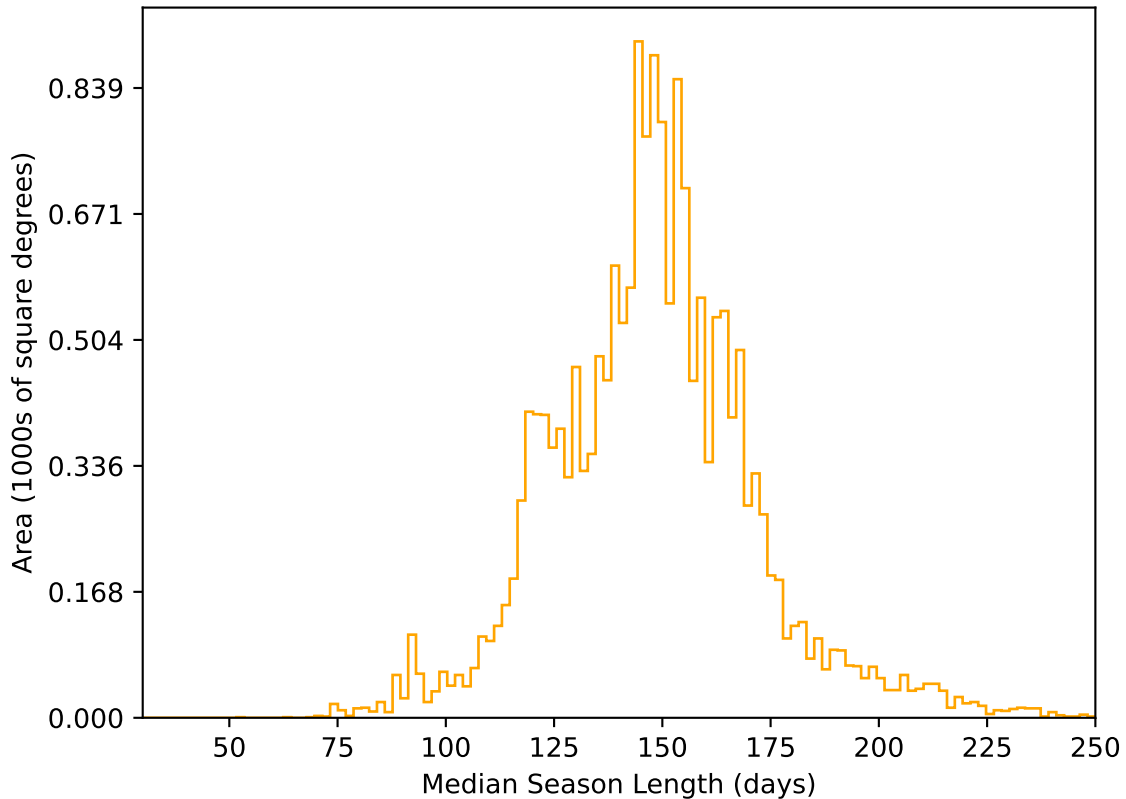
weather_cloudso6v3.4_10yrs WFD r band: Median Season Length
