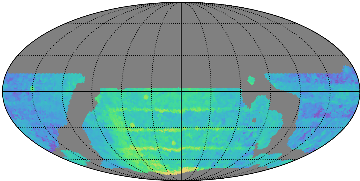
weather_cloudso6v3.4_10yrs WFD i band: Median Season Length
