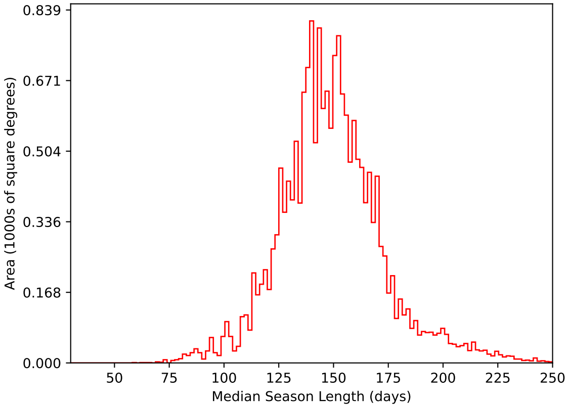
weather_cloudso6v3.4_10yrs WFD i band: Median Season Length
