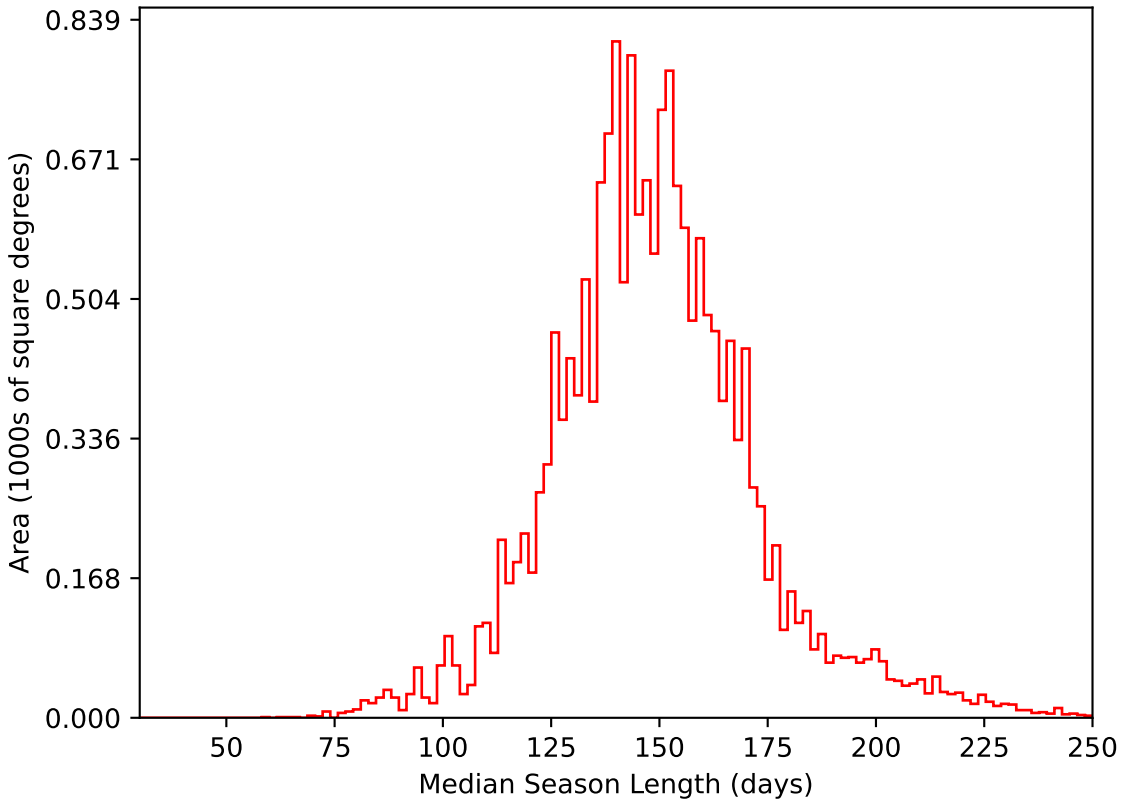
weather_cloudso6v3.4_10yrs WFD i band: Median Season Length
