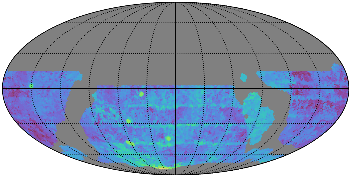
weather_cloudso6v3.4_10yrs WFD g band: Median Season Length
