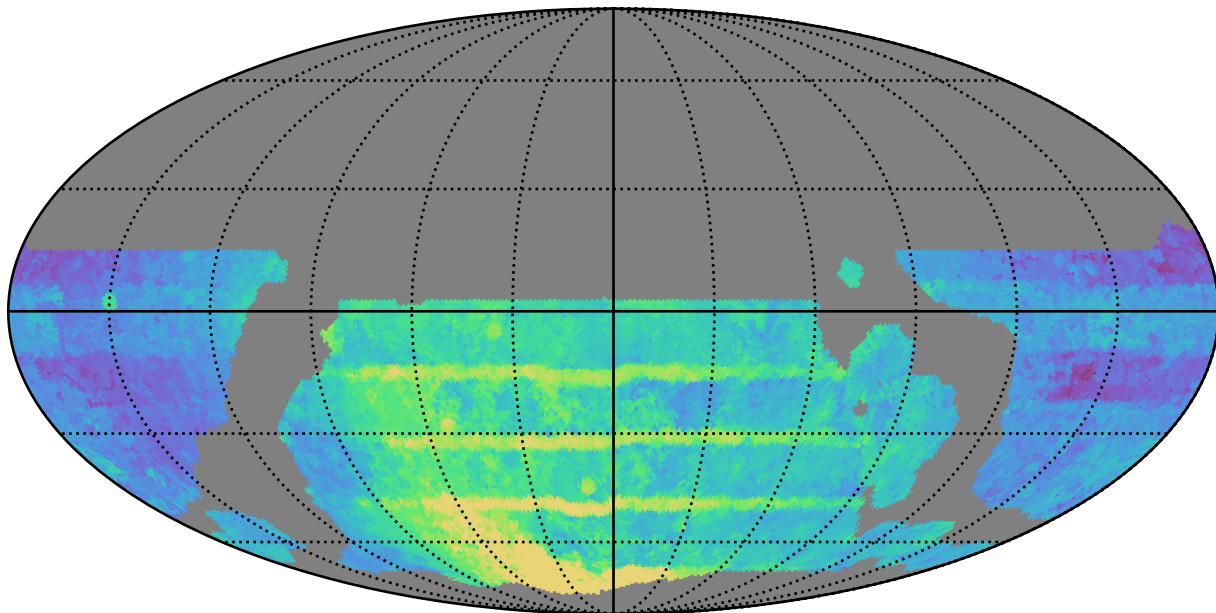
weather_cloudso6v3.4_10yrs WFD all bands: Median Season Length
