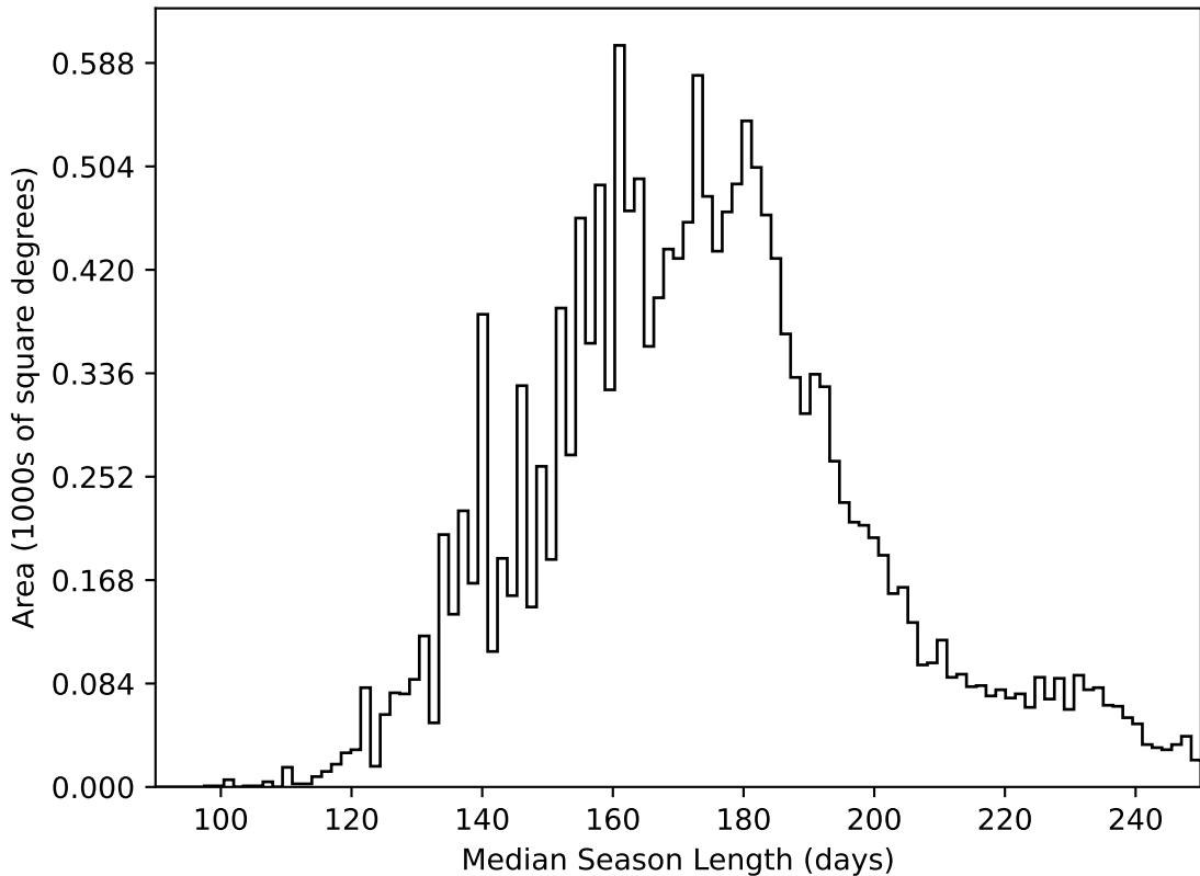
weather_cloudso6v3.4_10yrs WFD all bands: Median Season Length
