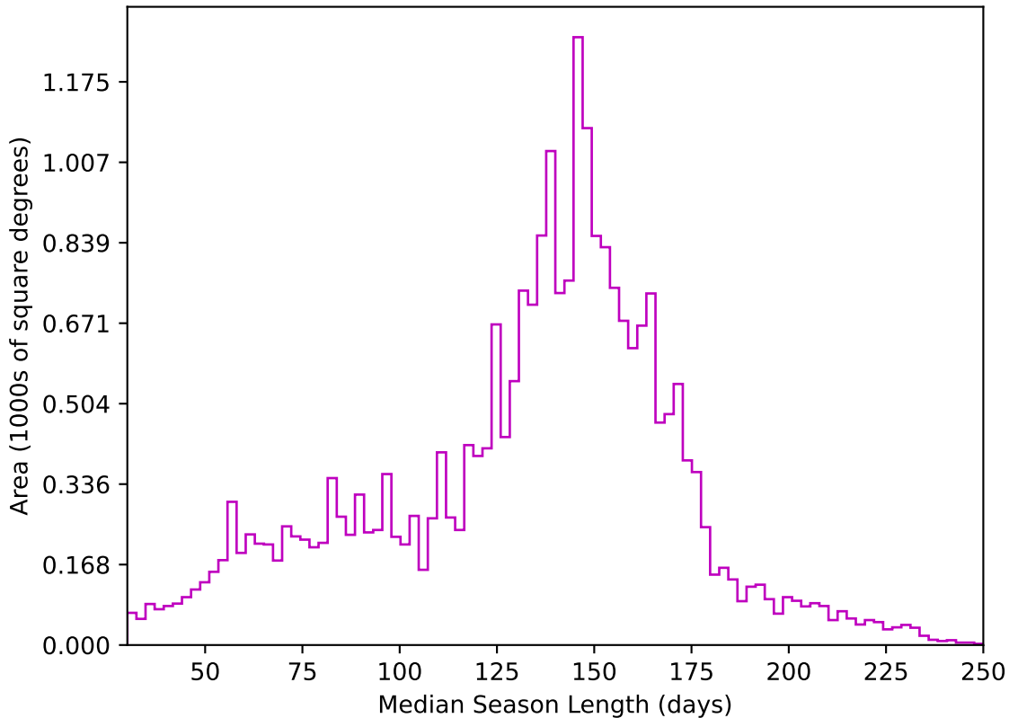
weather_cloudso6v3.4_10yrs All sky z band: Median Season Length
