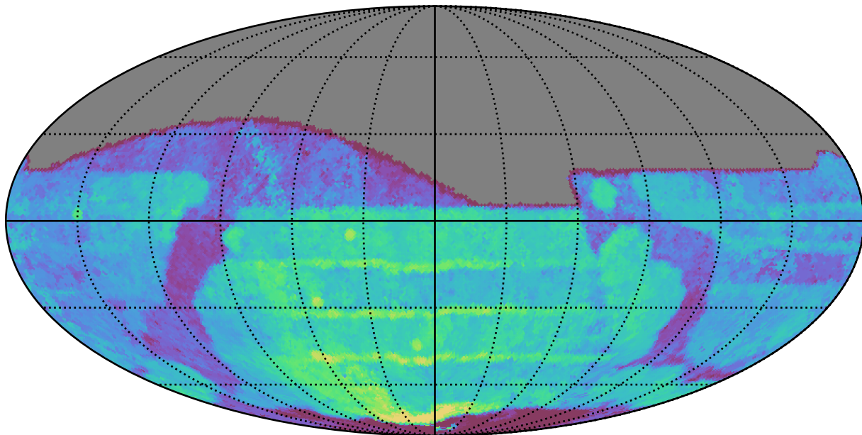
weather_cloudso6v3.4_10yrs All sky r band: Median Season Length
