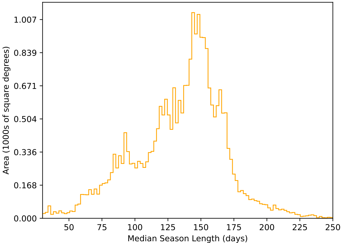
weather_cloudso6v3.4_10yrs All sky r band: Median Season Length
