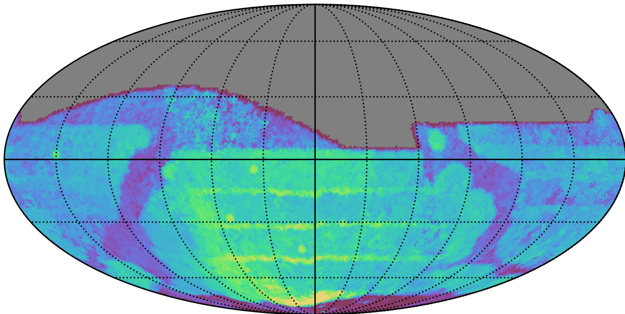
weather_cloudso6v3.4_10yrs All sky i band: Median Season Length
