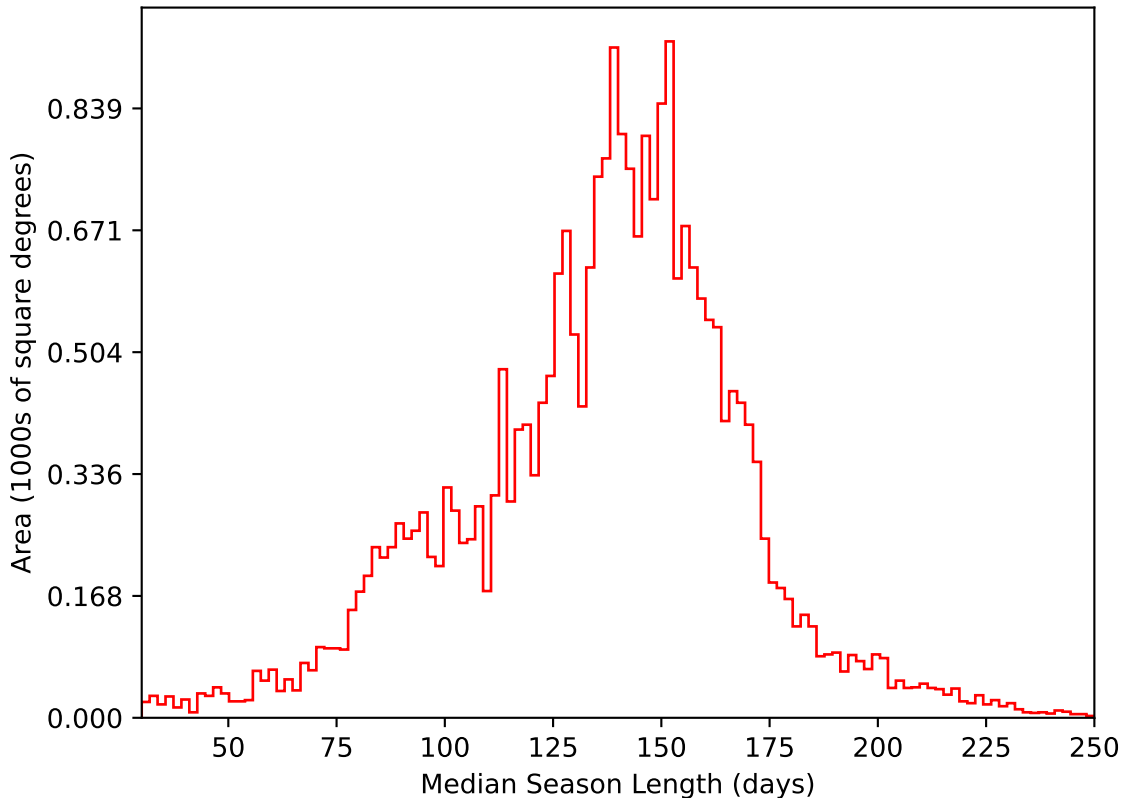
weather_cloudso6v3.4_10yrs All sky i band: Median Season Length
