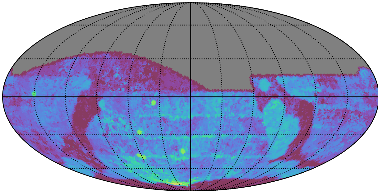
weather_cloudso6v3.4_10yrs All sky g band: Median Season Length
