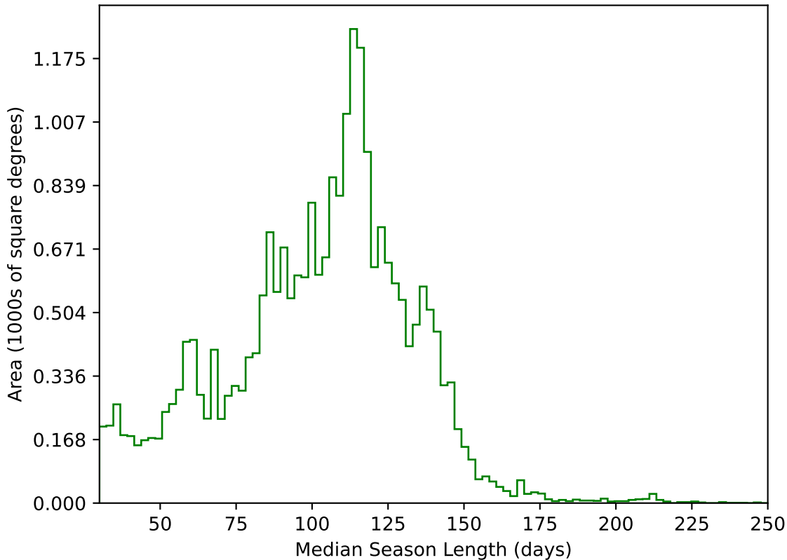
weather_cloudso6v3.4_10yrs All sky g band: Median Season Length
