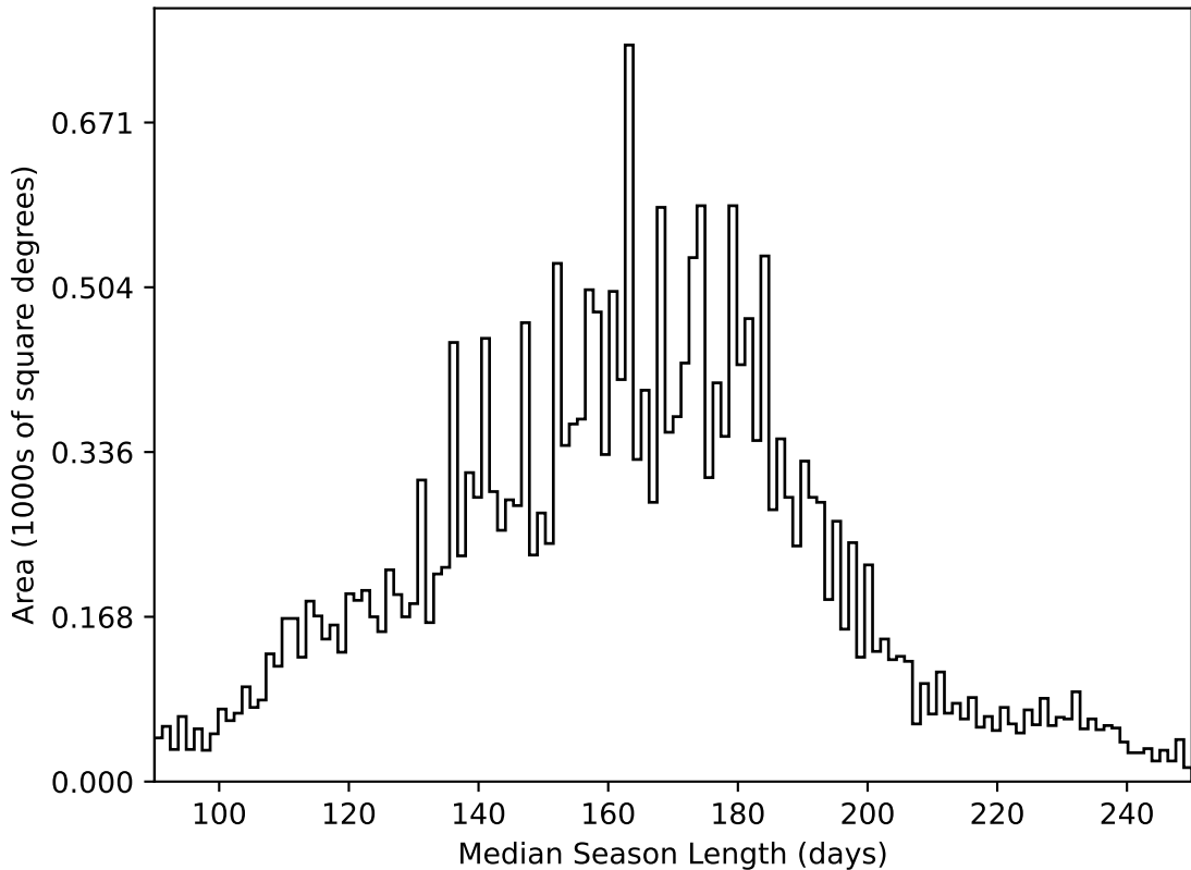
weather_cloudso6v3.4_10yrs All sky all bands: Median Season Length
