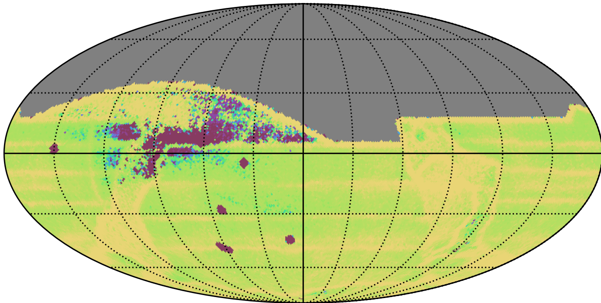
weather_cloudso6v3.4_10yrs All sky: Median Intra-Night Gap
