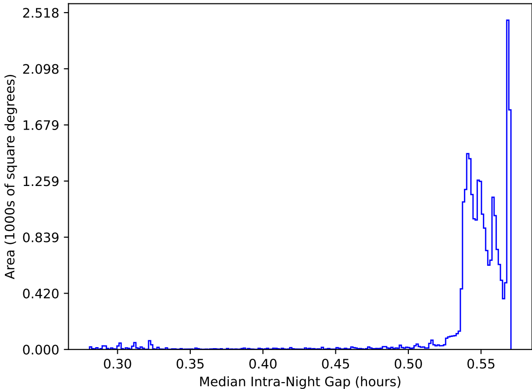
weather_cloudso6v3.4_10yrs All sky: Median Intra-Night Gap
