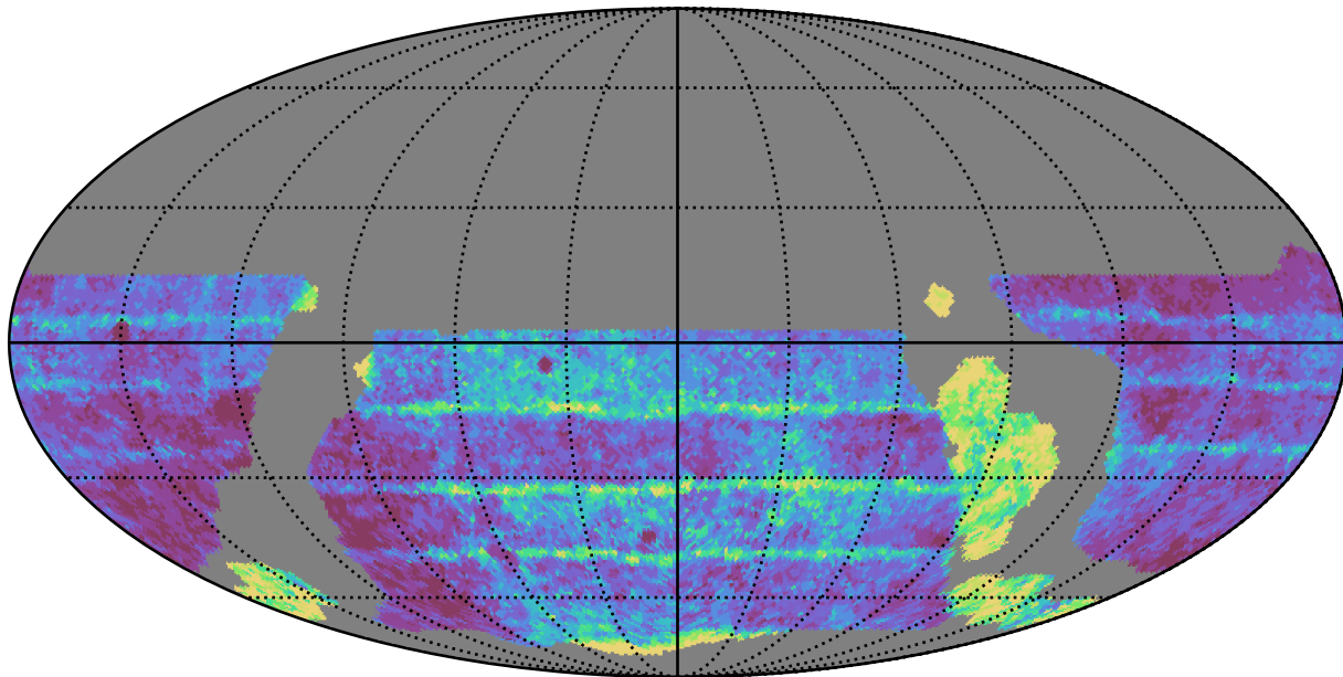
weather_cloudso6v3.4_10yrs WFD z band: Median Inter-Night Gap
