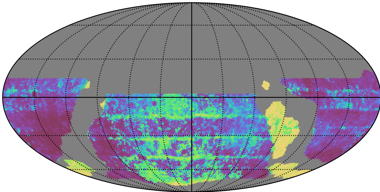
weather_cloudso6v3.4_10yrs WFD y band: Median Inter-Night Gap
