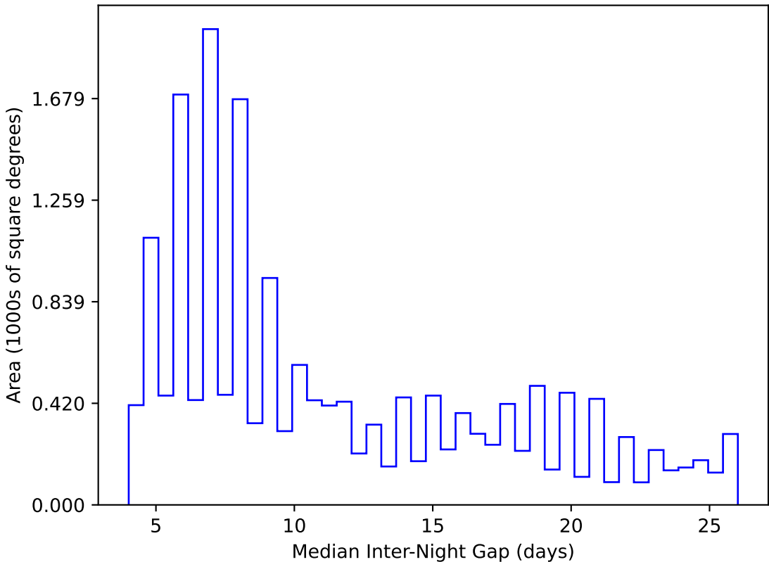
weather_cloudso6v3.4_10yrs WFD y band: Median Inter-Night Gap
