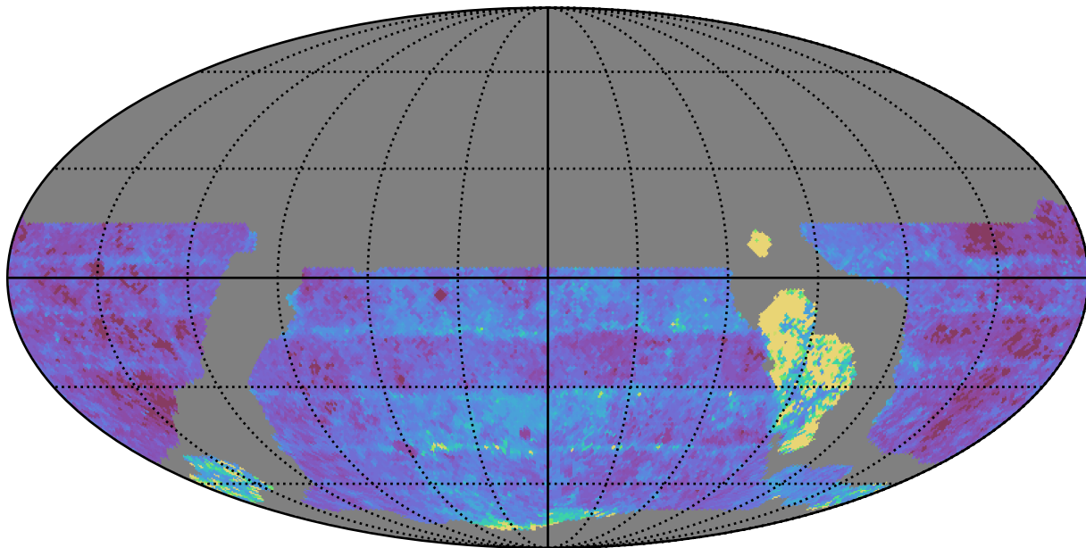
weather_cloudso6v3.4_10yrs WFD u band: Median Inter-Night Gap
