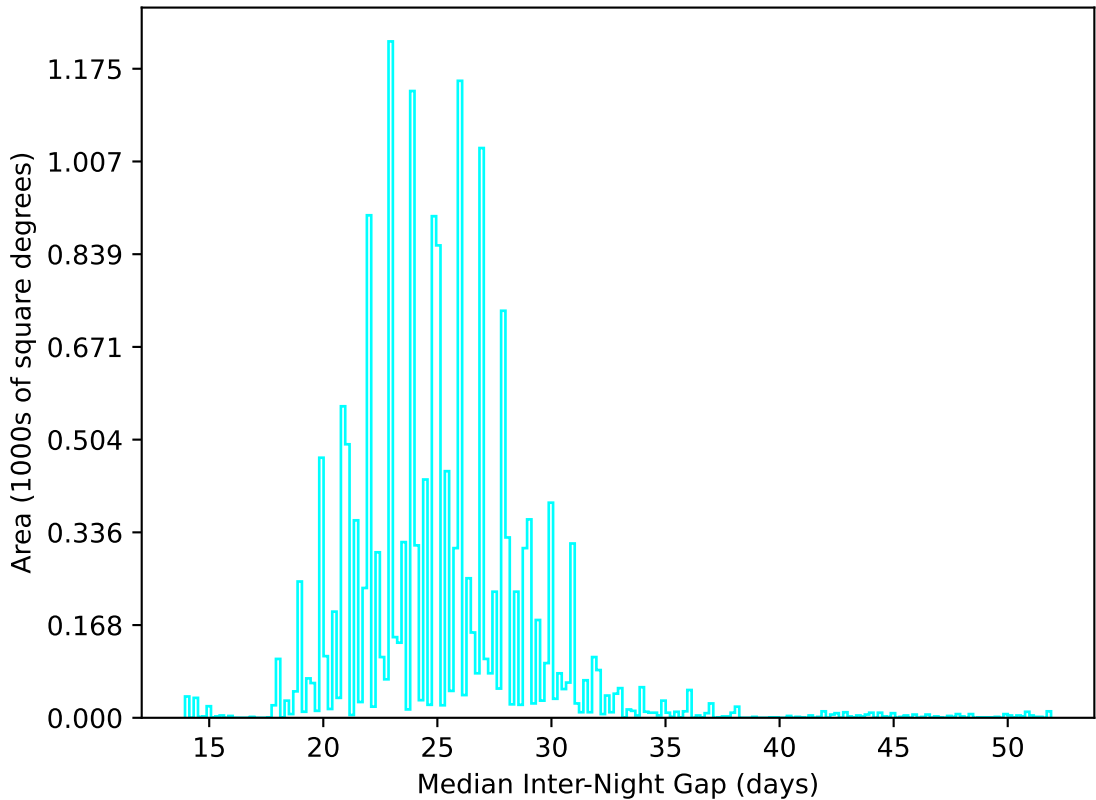
weather_cloudso6v3.4_10yrs WFD u band: Median Inter-Night Gap
